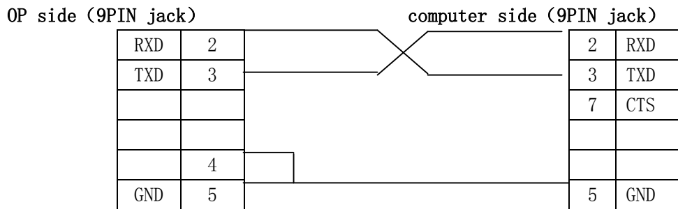
OP-SYS-CAB connecting graph: (V4.0):
