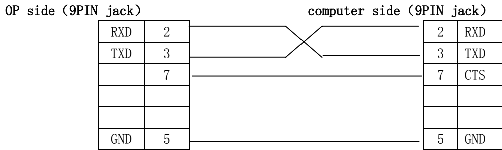
OP-SYS-CAB connecting graph
